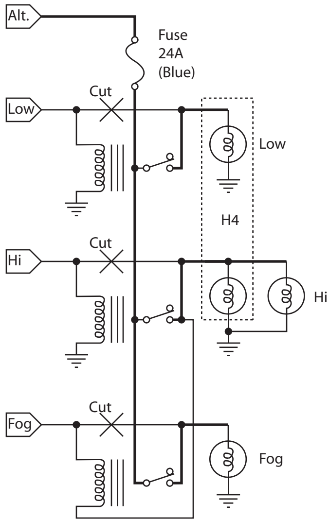
450 SL Head/Fog Light Relay System. (Typ. 1 side.)
